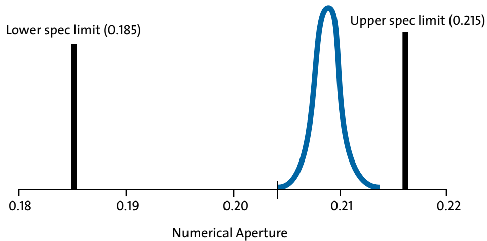
Numerical Aperture Distribution Data
