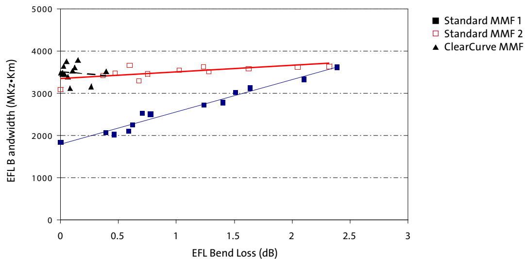
Impact of Macrobend Loss on Bandwidth
